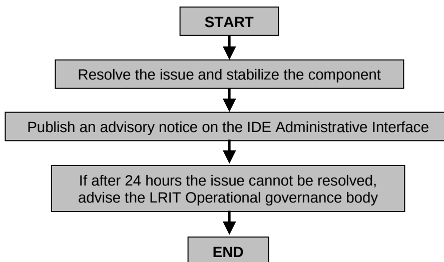
Figure 2 – Unforeseen events notification flow chart
